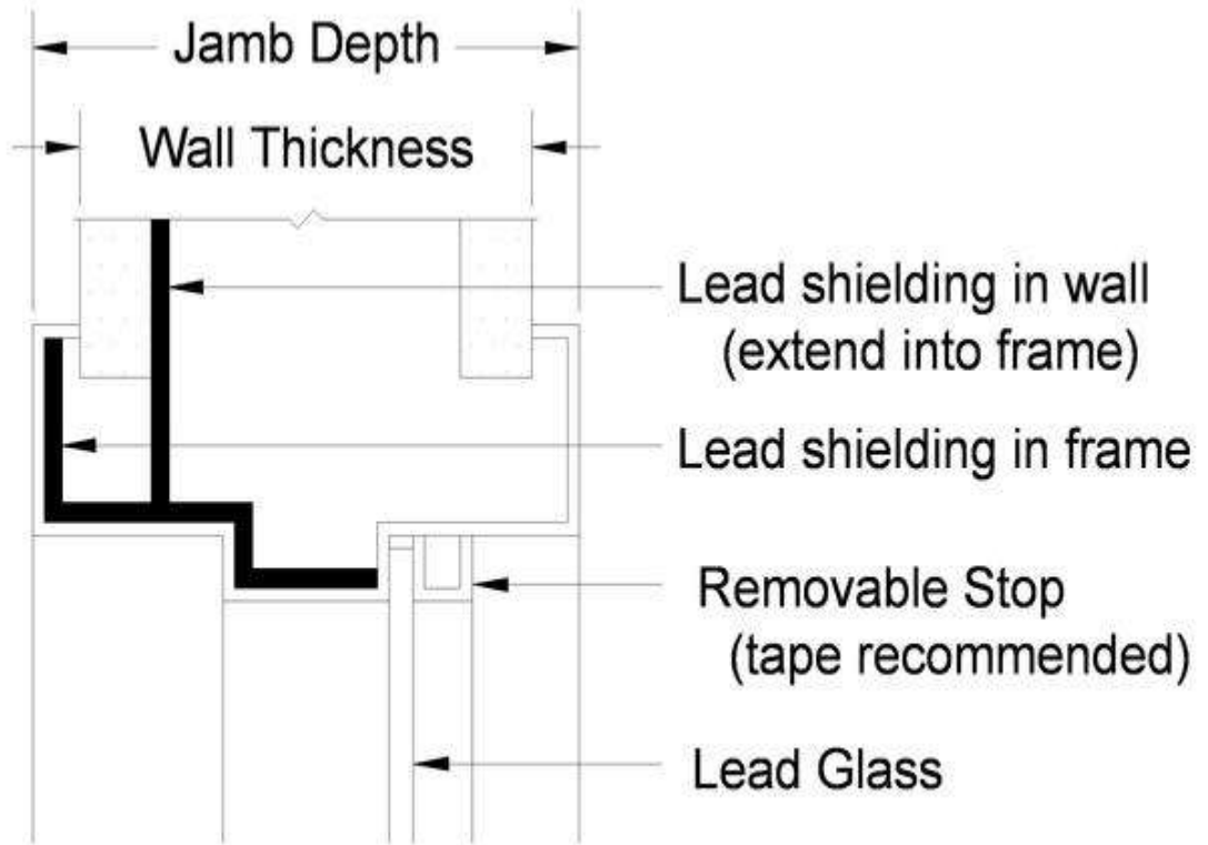
Lead Lined Window Frame Detail
