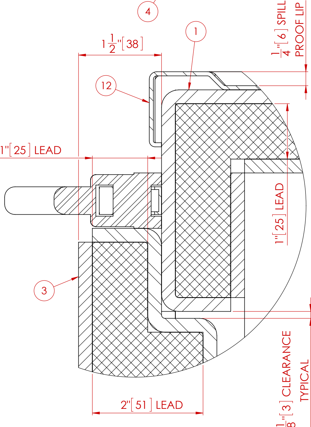
DETAIL B SCALE 1 : 1
