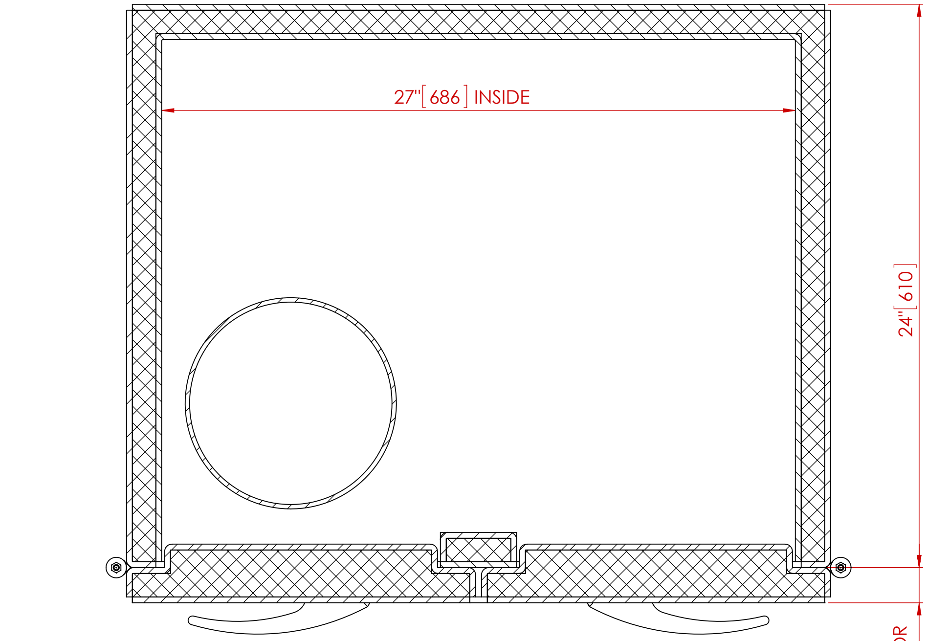
SECTION C-C
